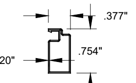
70 SCREEN FRAME
