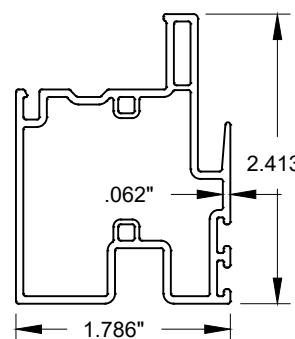
7 MEETING RAIL
