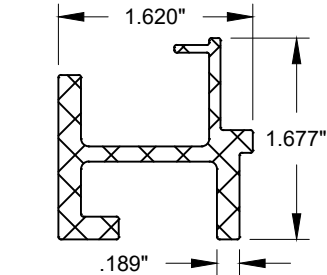
11 REINFORCEMENT (MEETING RAIL)
